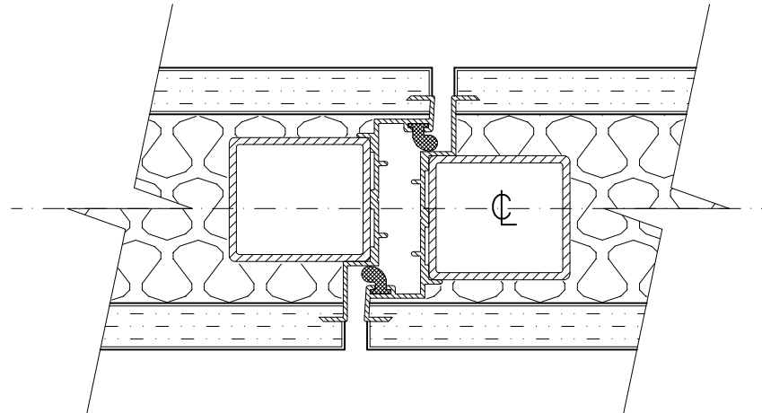
CLOSURE DETAIL
