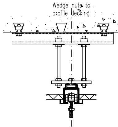
Typical Head Fixing Details
