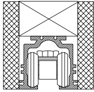
Alternative Head Detail With Pelmet.
