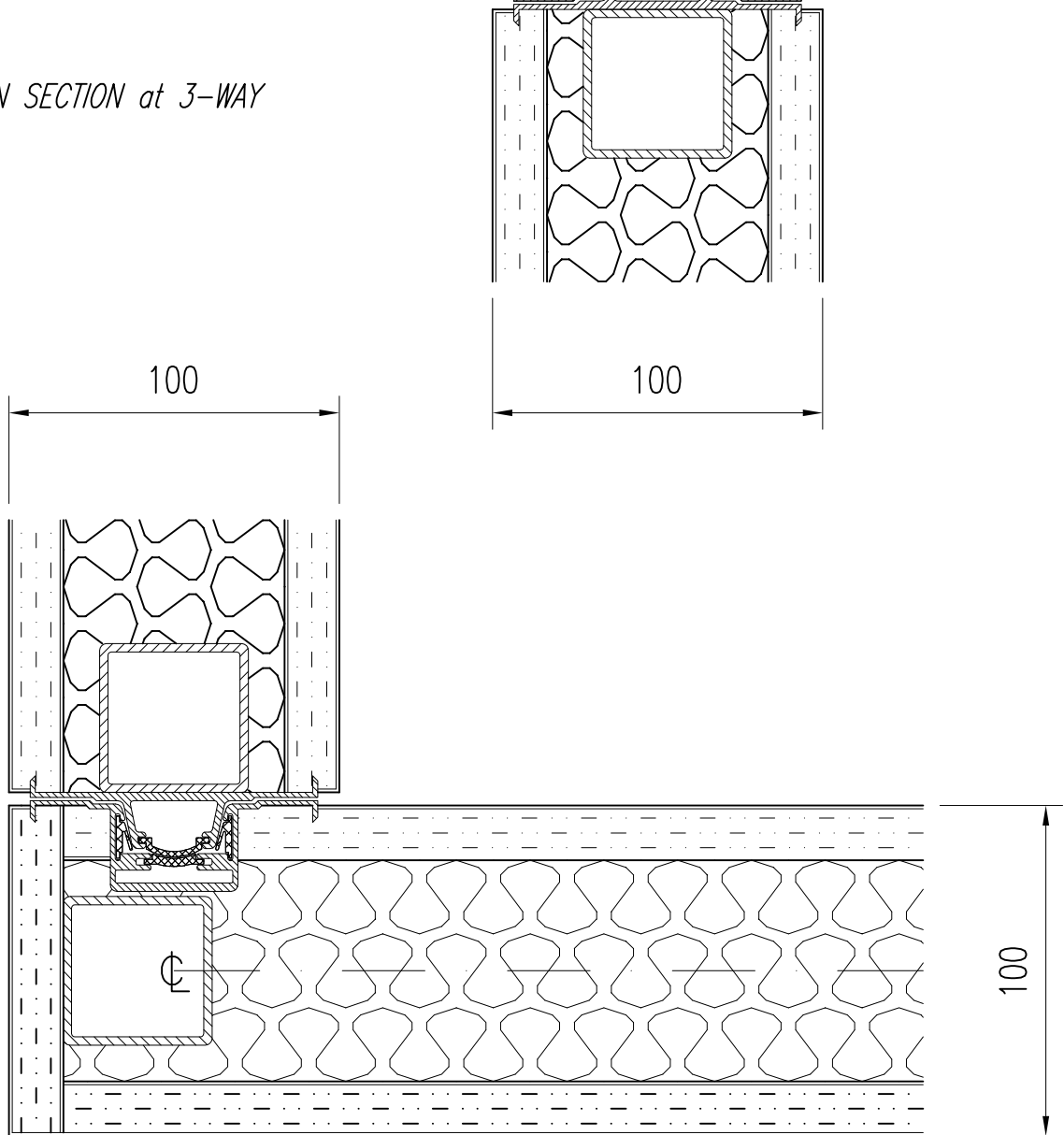
PLAN SECTION at CORNER
