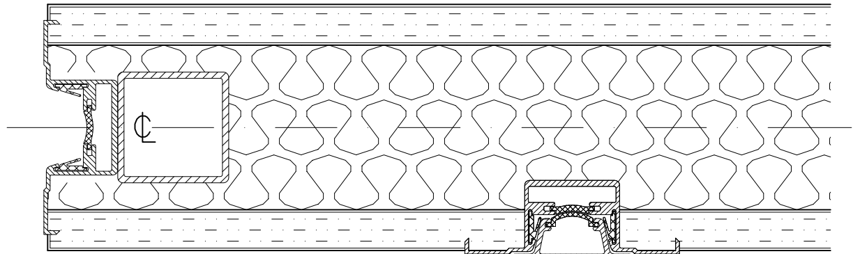
PLAN SECTION at 3-WAY
